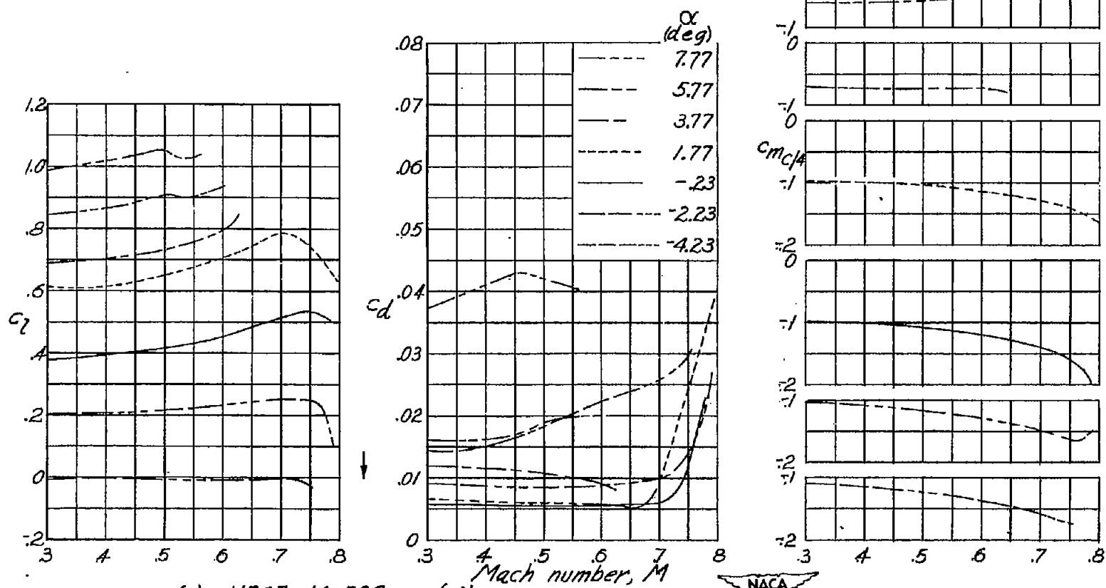
(c) NACA 16-509 airfoil. Figure 3.- Continued.
