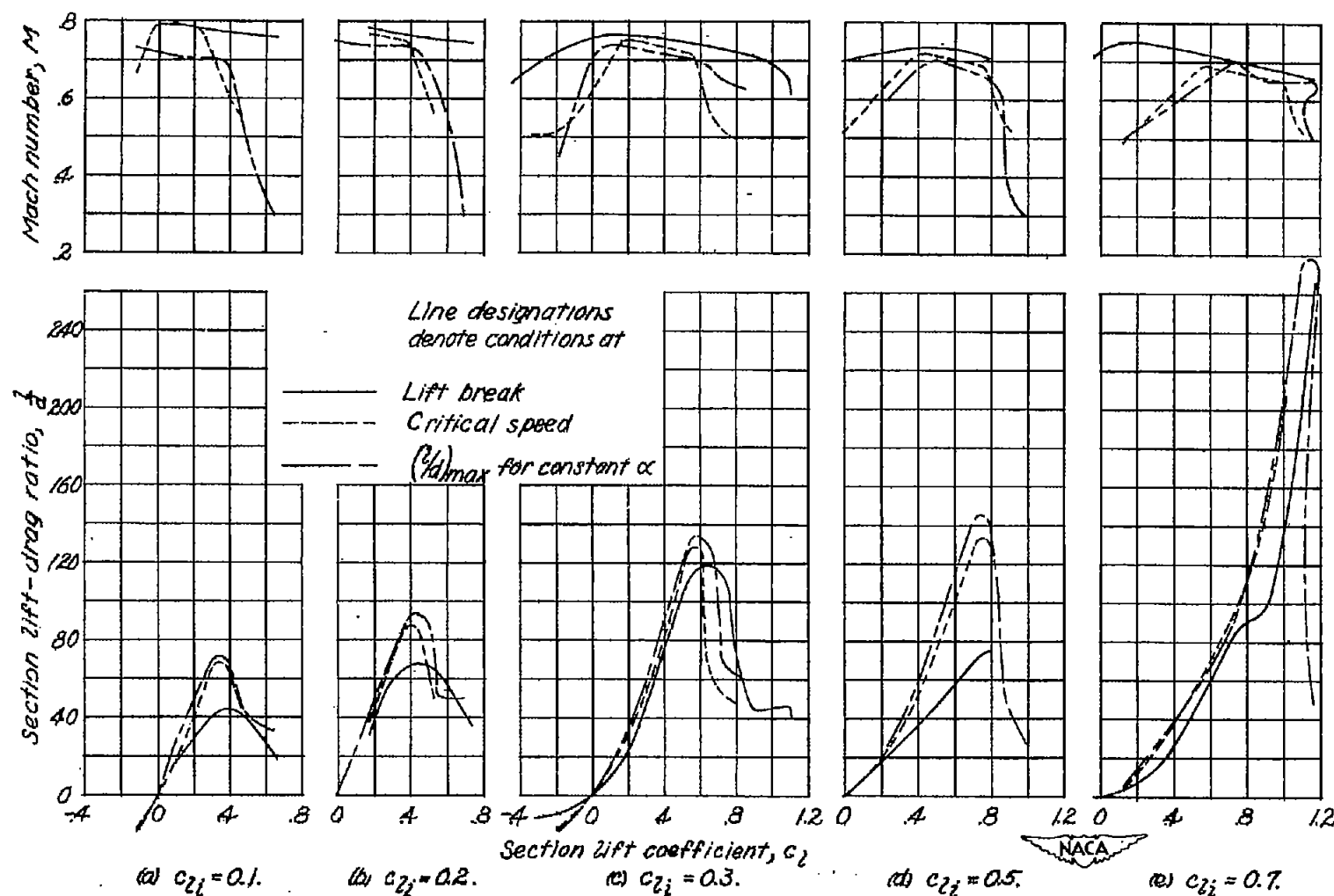
Figure 19.—Conditions for lift break, critical speed, and maximum lift-drag ratios for the NACA 16-X09 airfoils.
