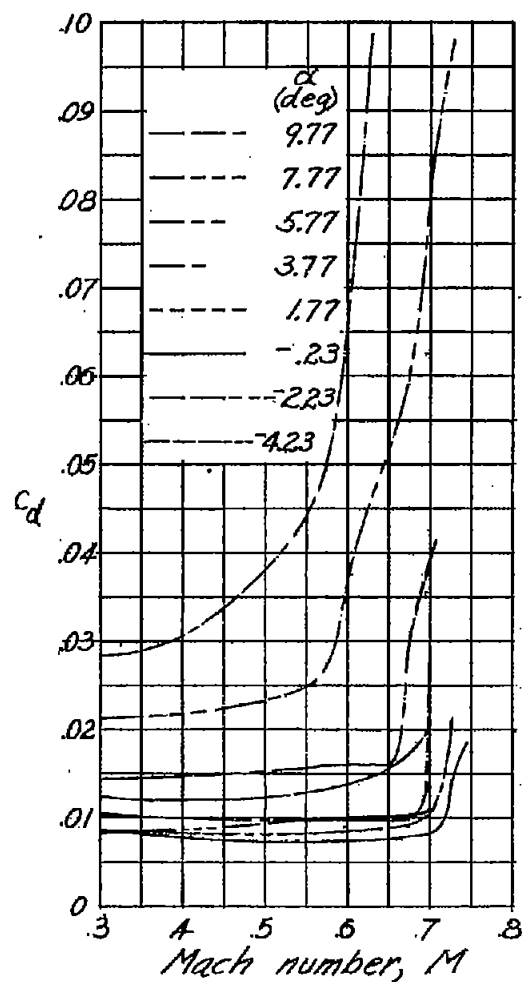
(k) NACA 16-315 airfoil. Figure 3.- Continued.
