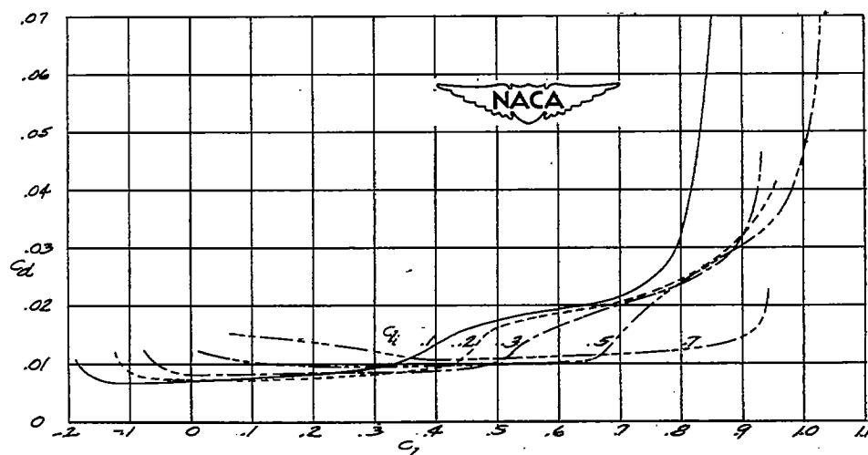
Figure 6. - Aerodynamic characteristics of NACA 16-X15 air foils.
