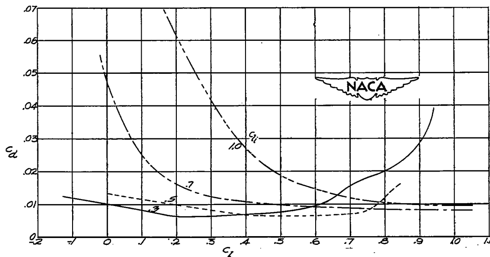
(C) M = 0.60 , Figure 5.-Continued.
