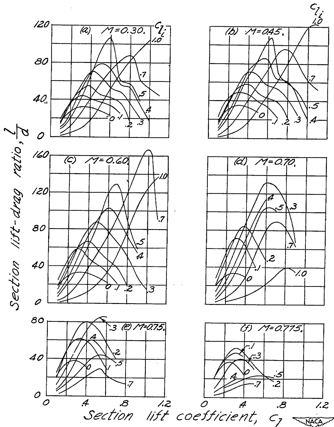
Figure 11.—Variation of section lift-drag ratio with section lift coefficient for NACA 16-X09 airfoils.
