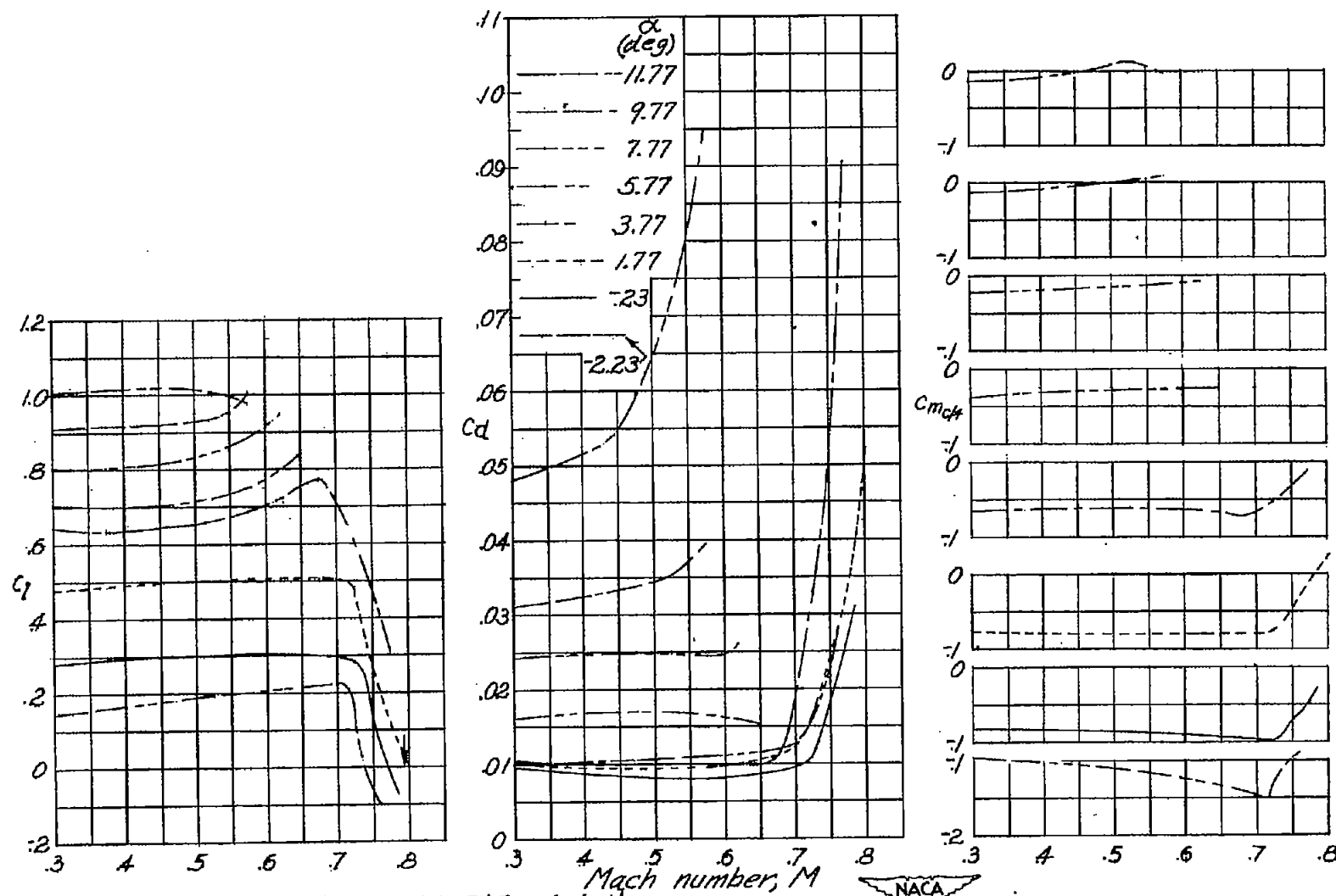
(q) NACA 16-515 airfoil. Figure 3.- Continued.
