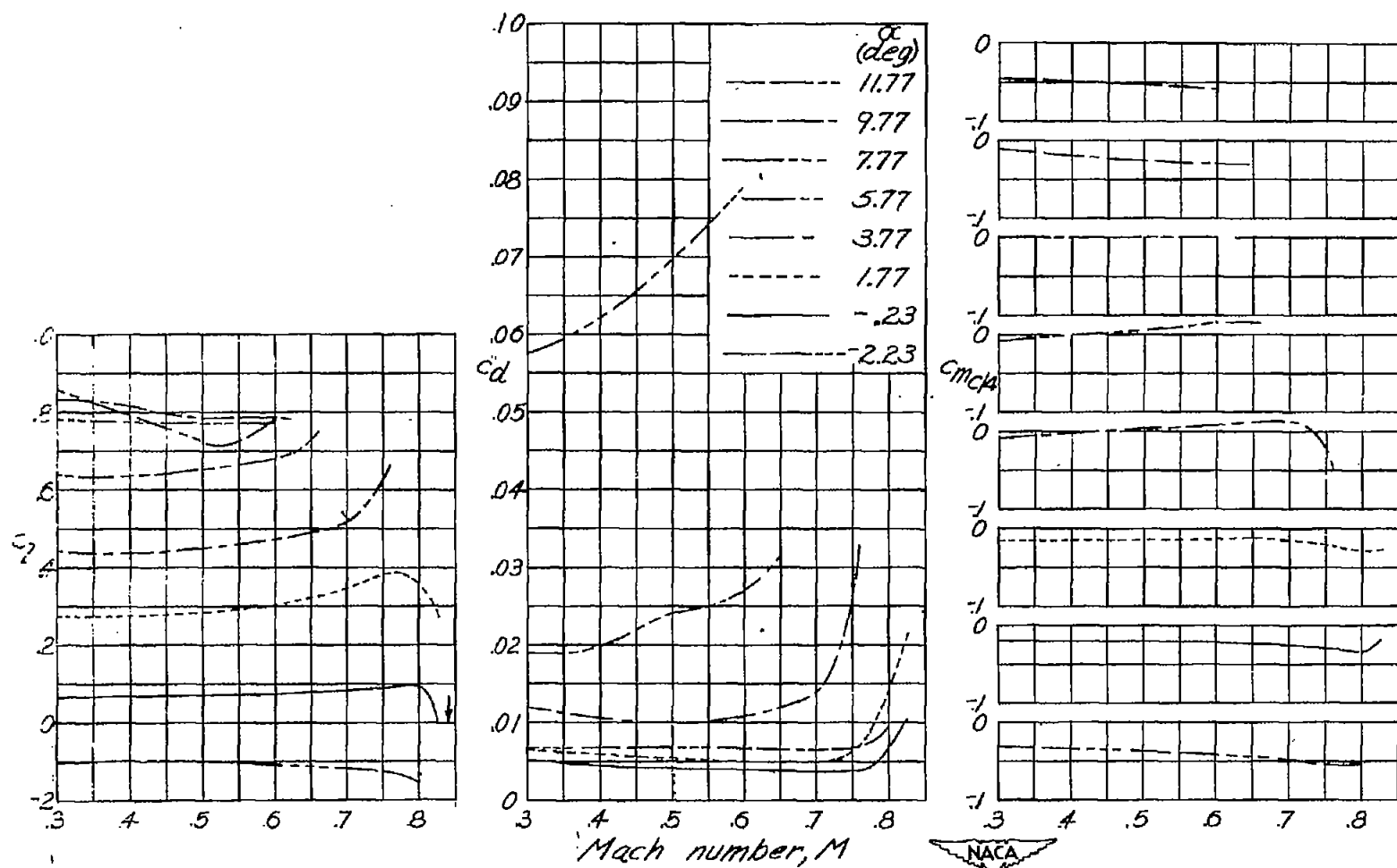
(c) NACA 16-109 airfoil. Figure 3.- Continued.
