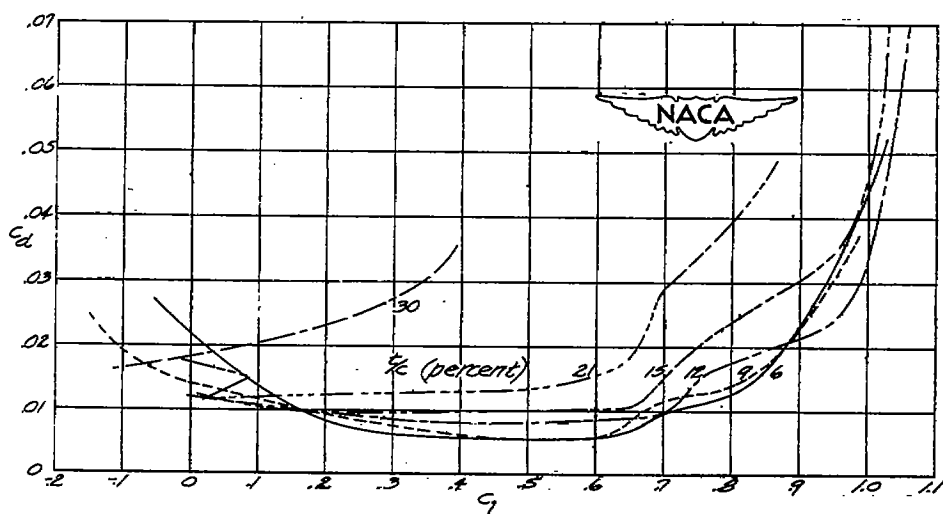
(a) M = 0.50 . Figure 9.- Aerodynamic characteristics of NACA 16-5XX airfoils.
