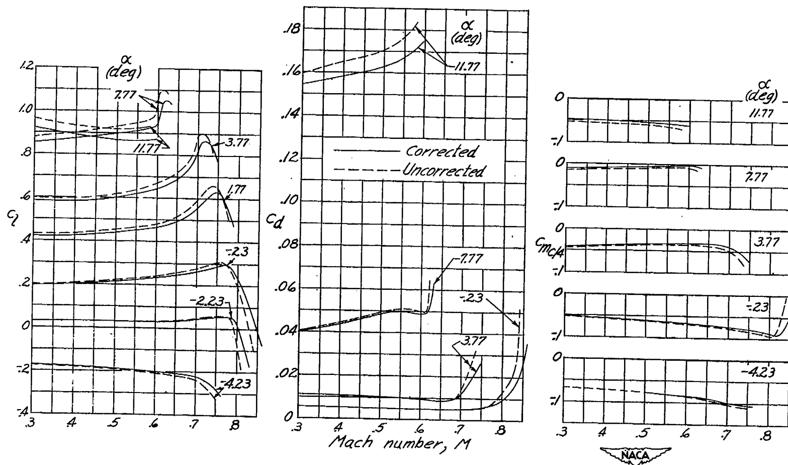
Figure 2.—A comparison of corrected and uncorrected data for the NACA 16-309 airfoil. (Corrections were determined by the method of reference 5.)
