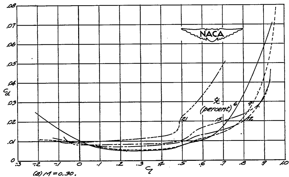
Figure 8.- Aerodynamic characteristics of NACA 16-3XX airfoils.
