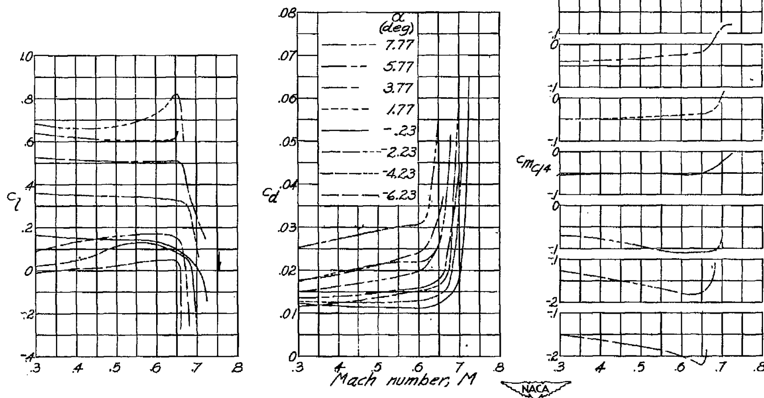
(r) NACA 16-521 airfoil. Figure 3.-Continued.
