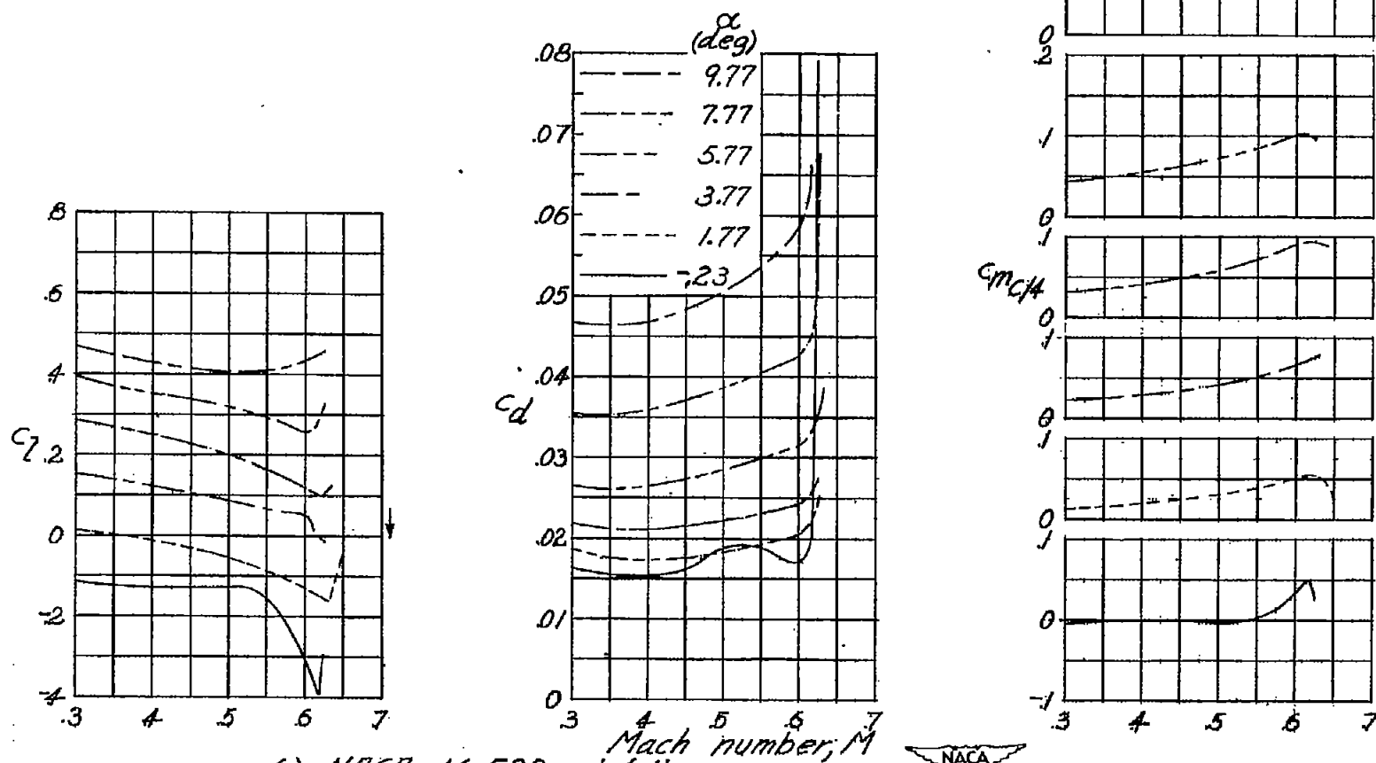
(5) NACA 16-530 airfoil. Figure 3.- Continued.
