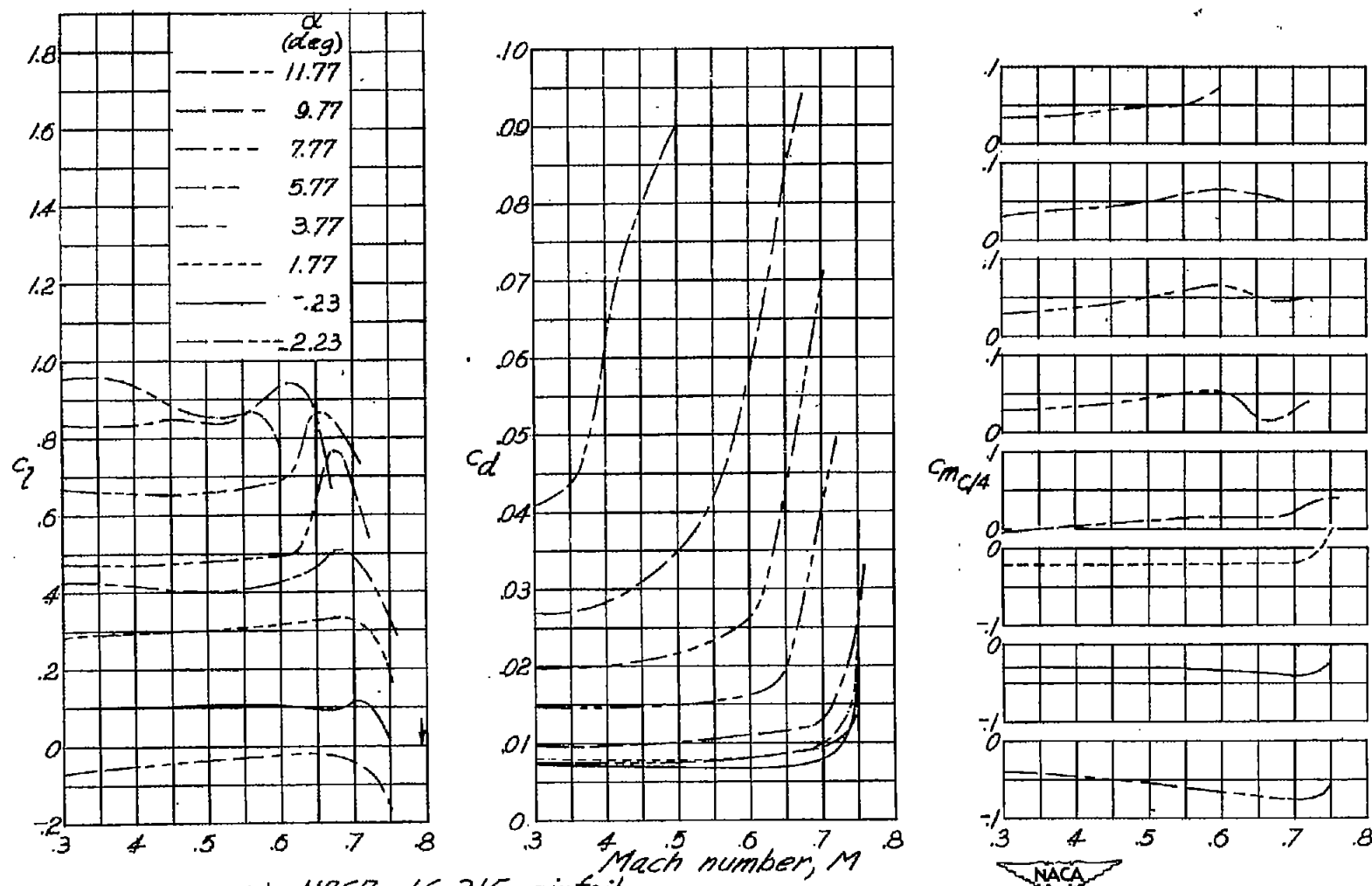
(9) NACA 16-215 airfoil. Figure 3.- Continued.
