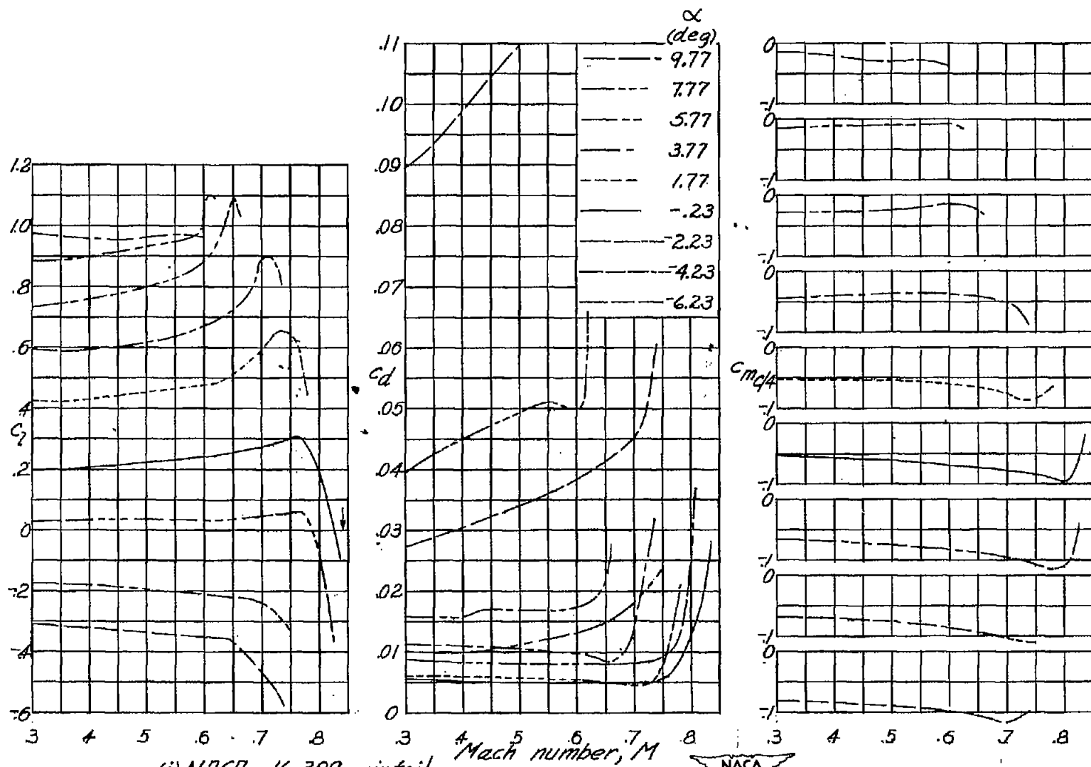
(1) NACA 16-309 airfoil. Figure 3.- Continued.
