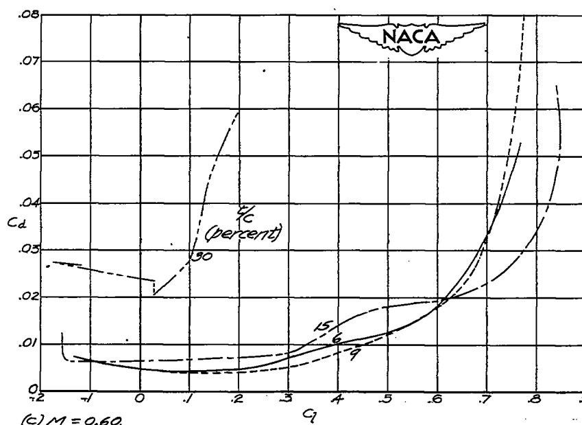
(c) M = 0.60 . Figure 7.- Continued.
