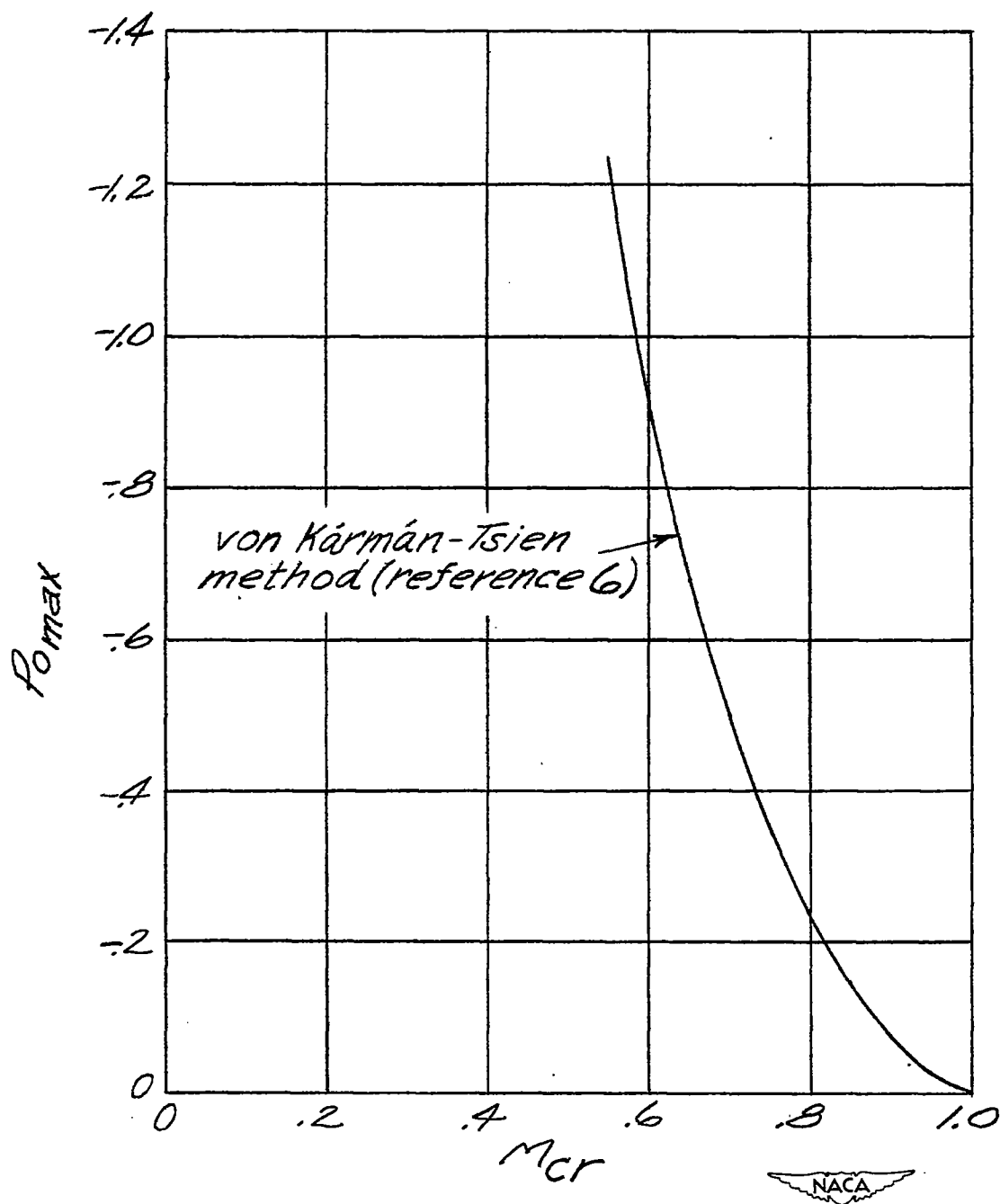
Figure 16.- Variation with critical Mach number of the maximum incompressible pressure coefficient.
