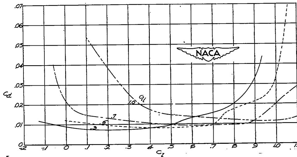
Figure 5. - Aerodynamic characteristics of NACA 16-X12 airfoils.
