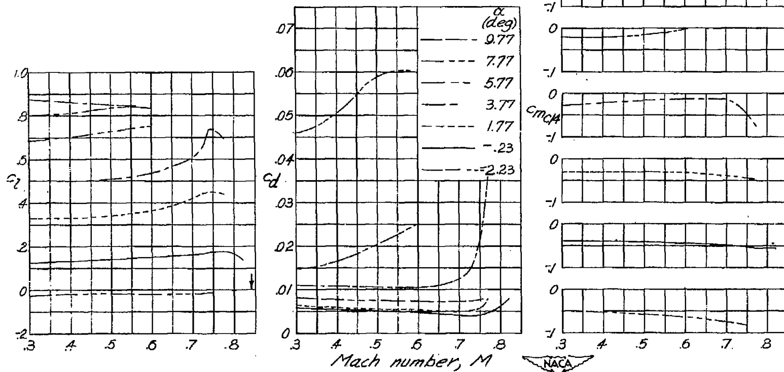
(f) NACA 16-209 airfoil. Figure 3.-Continued.
