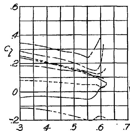
(e) NACA 16-130 airfoil. Figure 3.-Continued.
