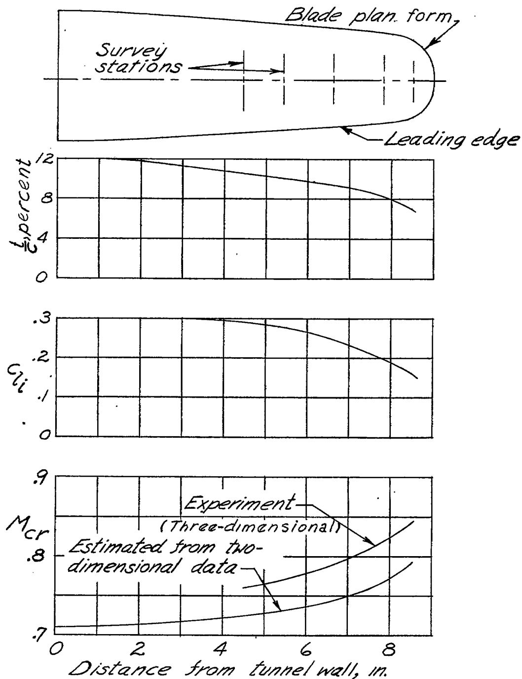
Figure 18.-Measurements near the tip of an untwisted propeller blade. \alpha = 0^\circ .
