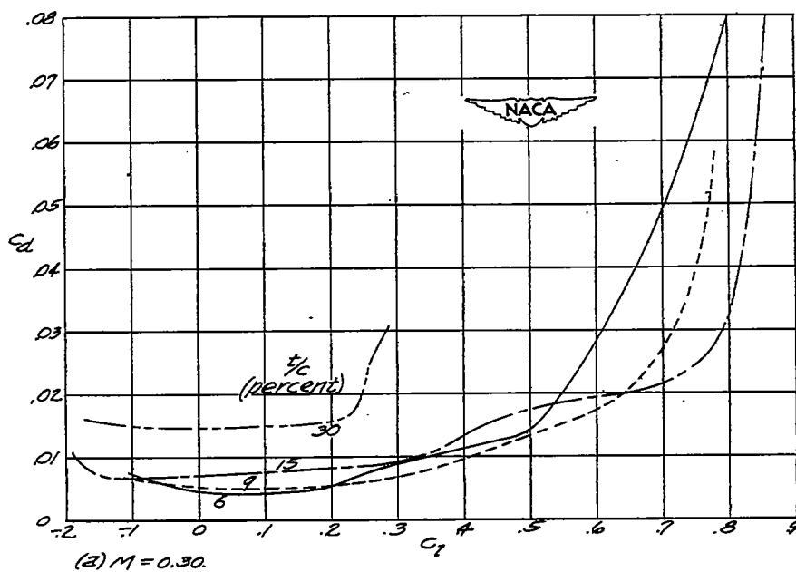
Figure 7.- Aerodynamic characteristics of NACA 16-1XX airfoils
