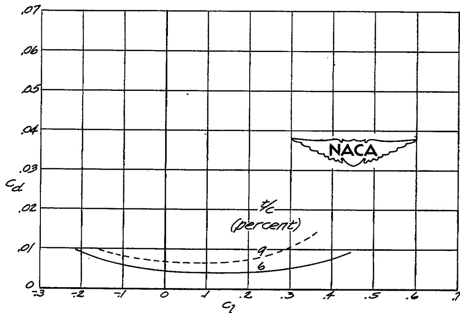
(f) M = 0.80 . Figure 7.- Concluded.
