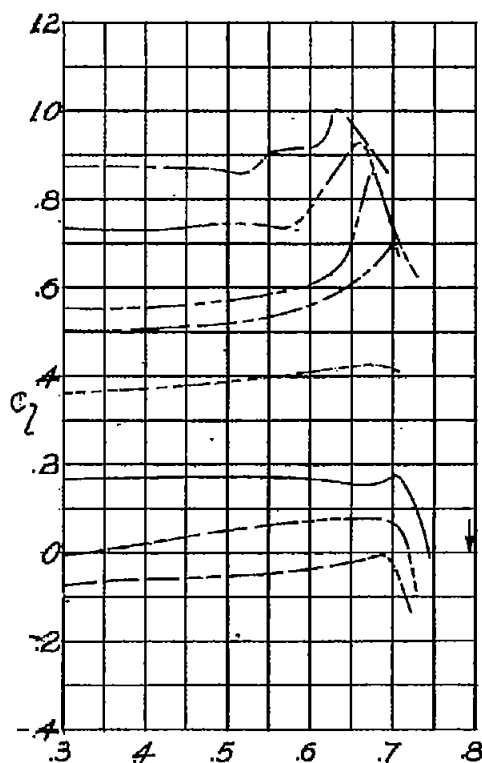
(k) NACA 16-315 airfoil. Figure 3.- Continued.
