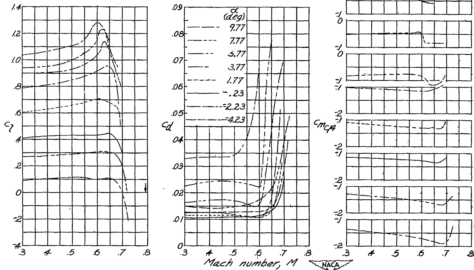
(v) NACA 16-715 airfoil. Figure 3.-Continued.
