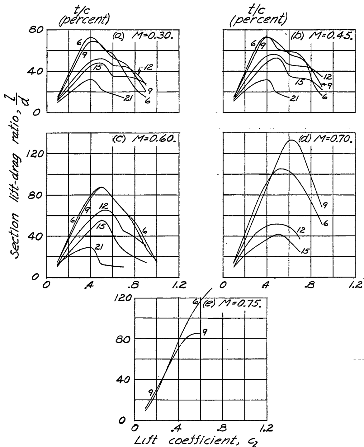
Figure 14.—Variation of section lift-drag ratio with section lift coefficient for NACA 16-3XX airfoils.
