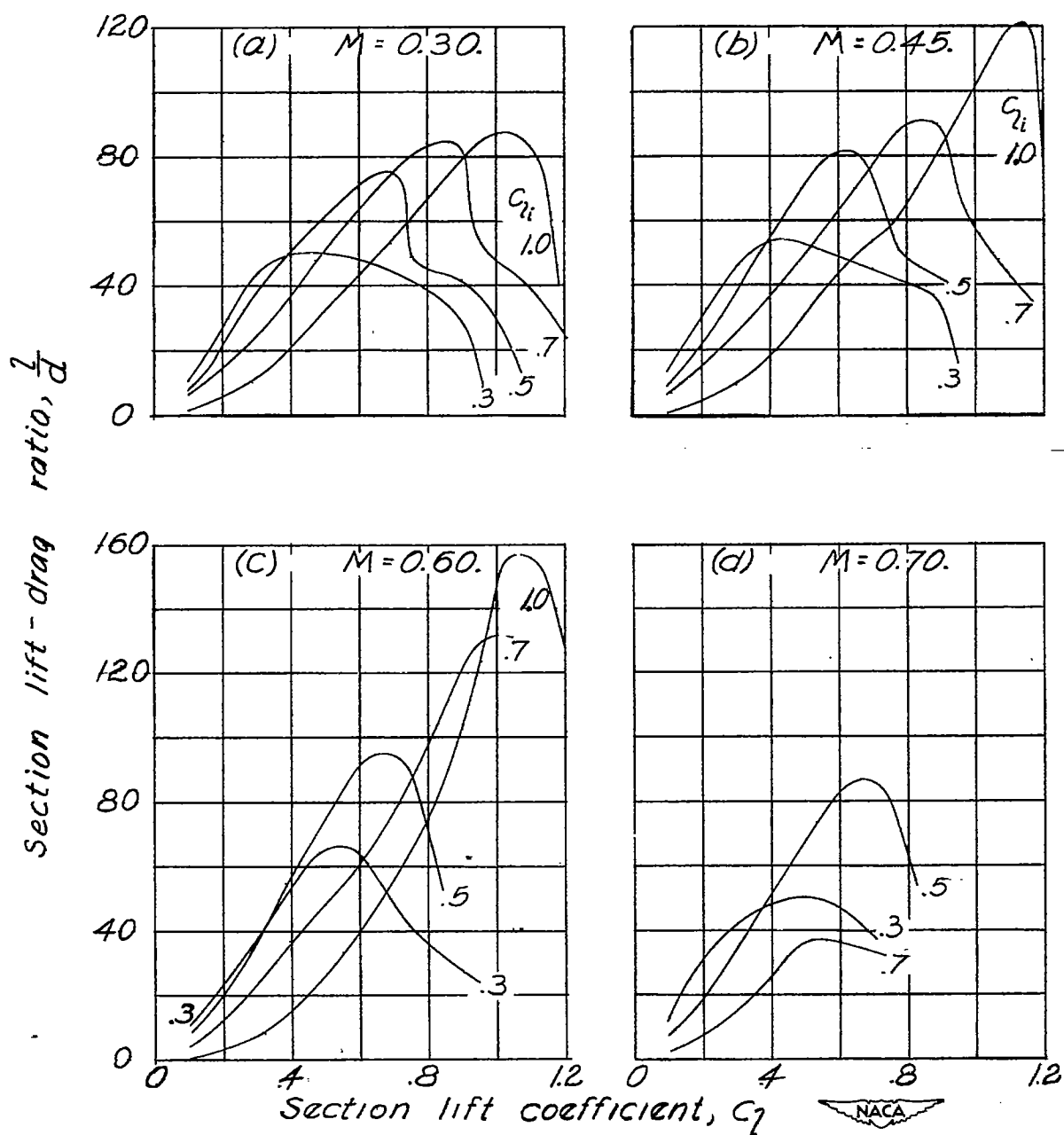
Figure 12.— Variation of section lift-drag ratio with section lift coefficient for NACA 16-X12 airfoils.
