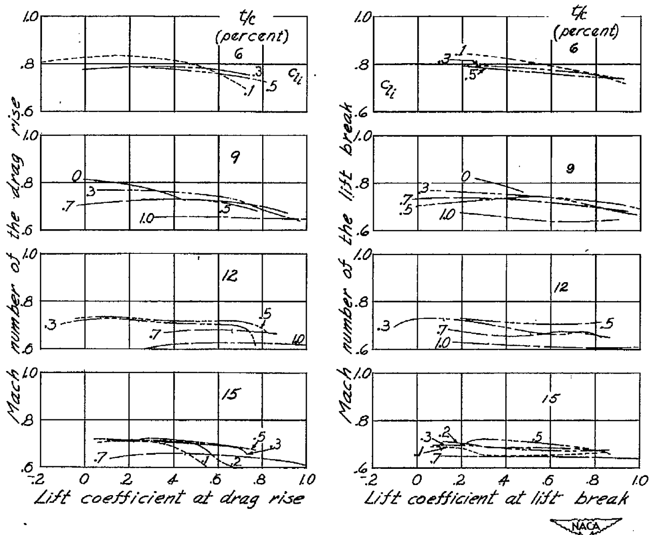
Figure 20.—Lift-break and drag-rise characteristics of various NACA 16-series airfoils.
