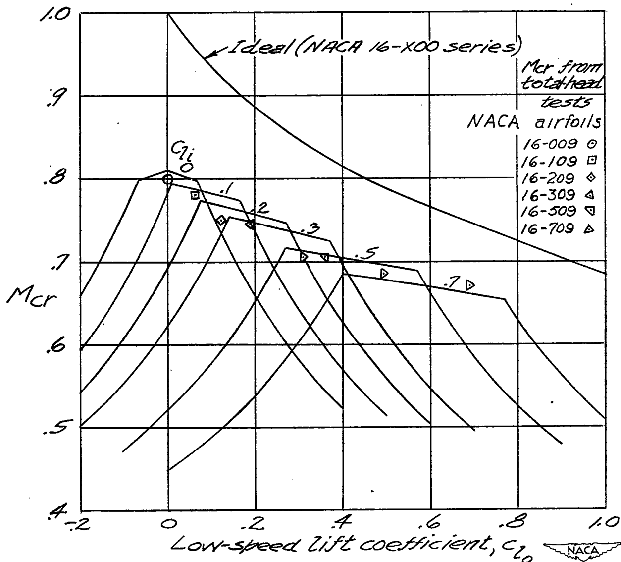
(d) Theoretical variation of critical Mach number with low-speed lift coefficient for NACA 16-x09 airfoils of various cambers.
