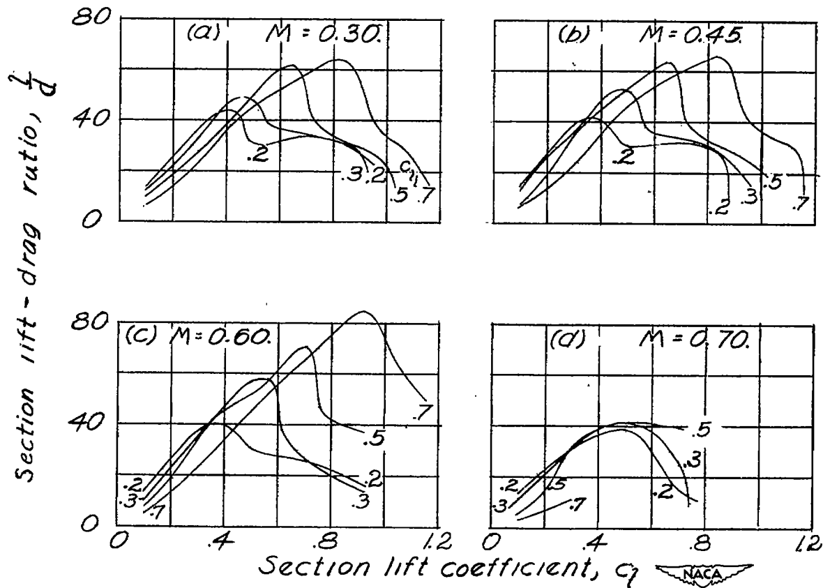
Figure 13.— Variation of section lift-drag ratio with section lift coefficient for NACA 16-X15 airfoils.
