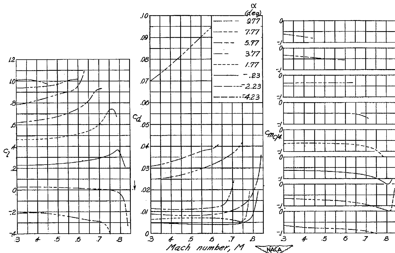
(h) NACA 16-306 airfoil. Figure 3.- Continued.
