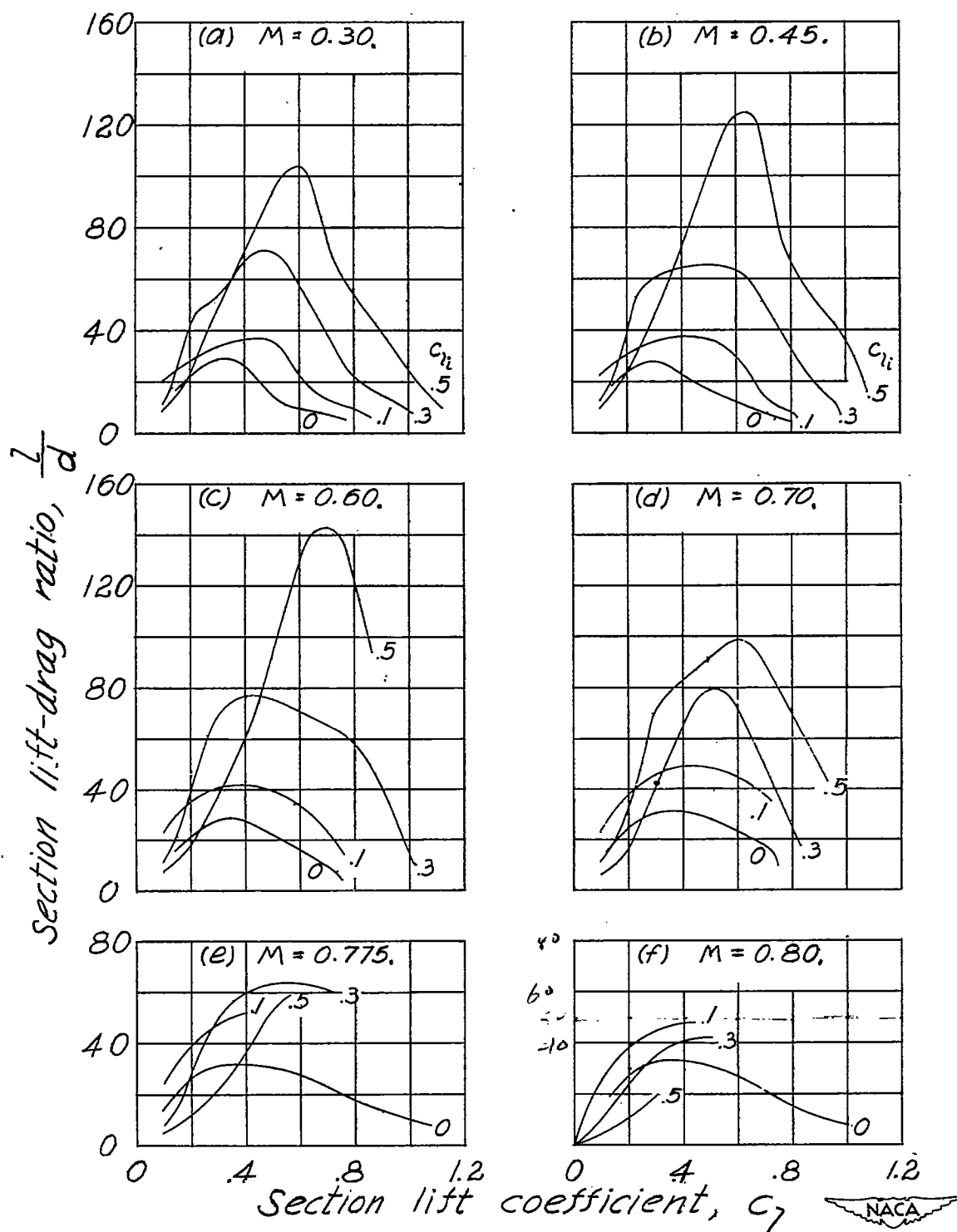
Figure 10.—Variation of section lift-drag ratio with section lift coefficient for NACA 16-X06 airfoils.
