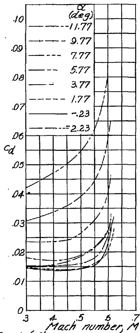
(e) NACA 16-130 airfoil. Figure 3.-Continued.
