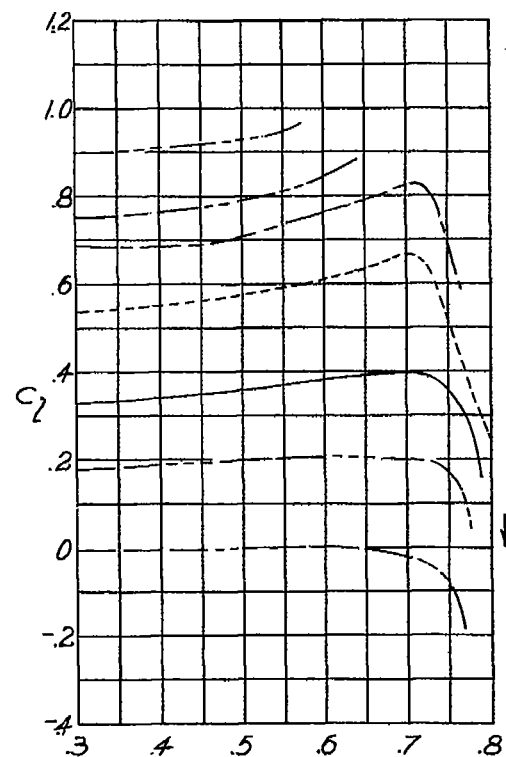
(p) NACA 16-512 airfoil. Figure 3-Continued.
