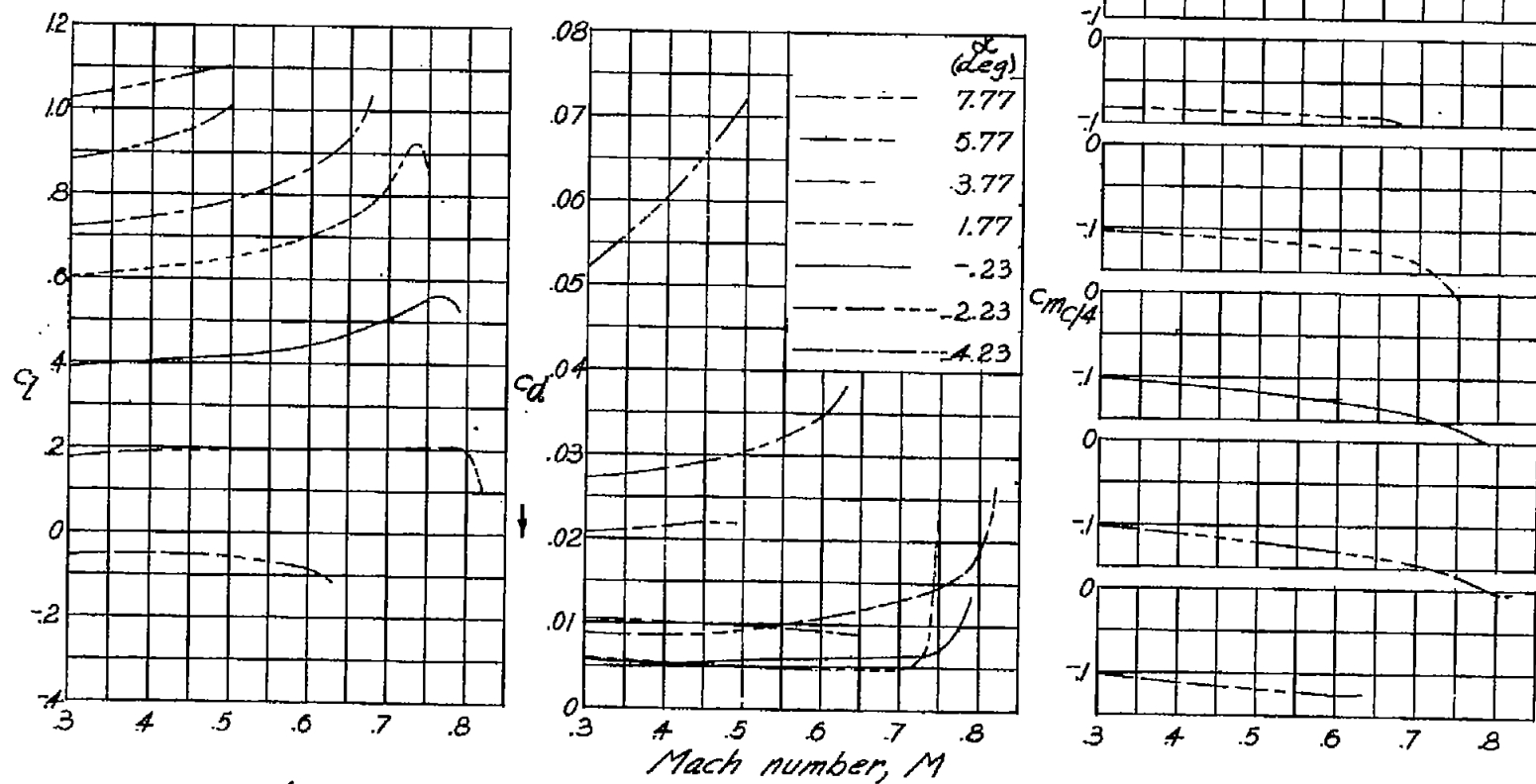
(n) NACA 16-506 airfoil. Figure 3.- Continued.
