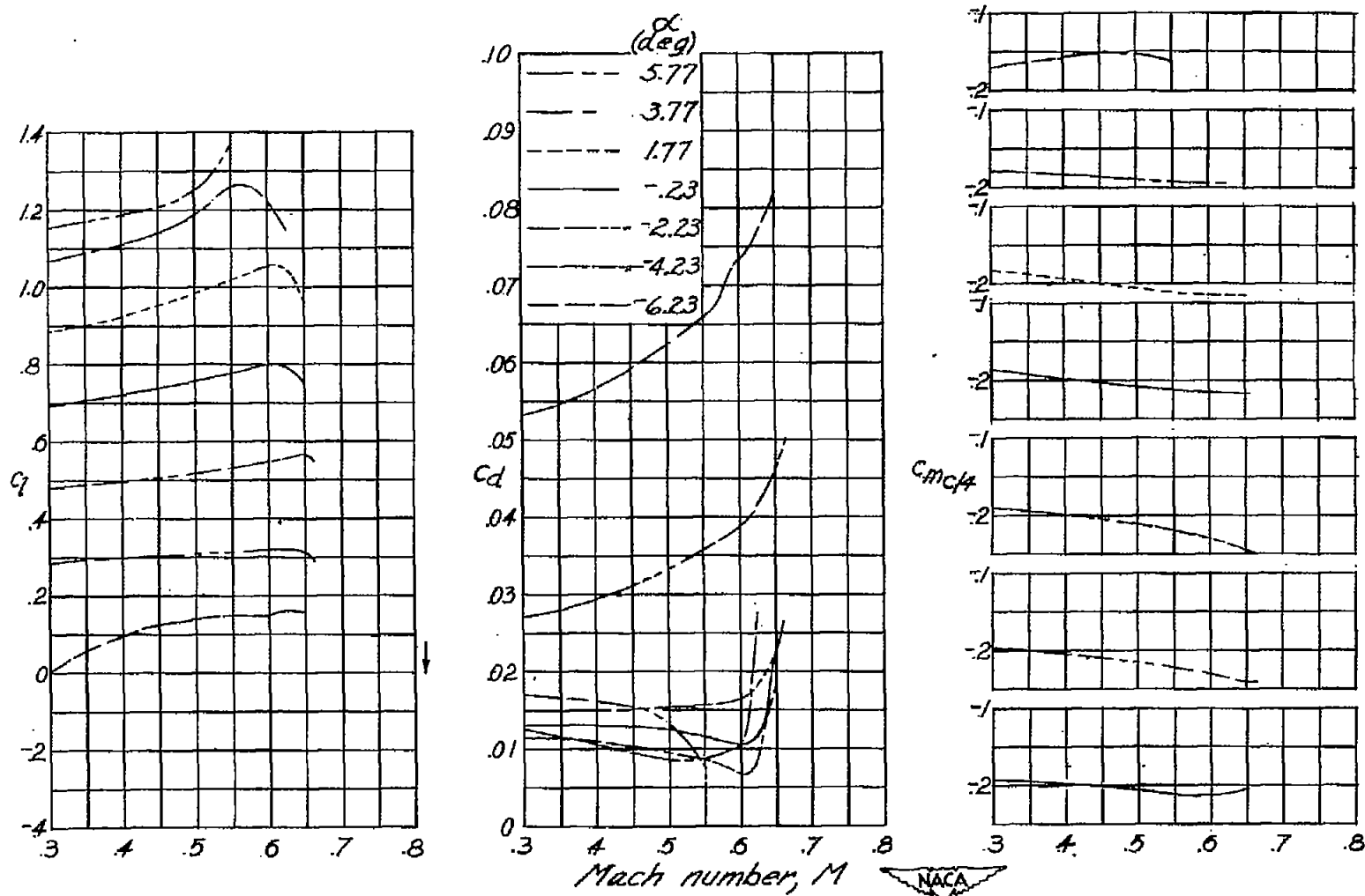
(X) NACA 16-1012 airfoil. Figure 3.- Concluded.
