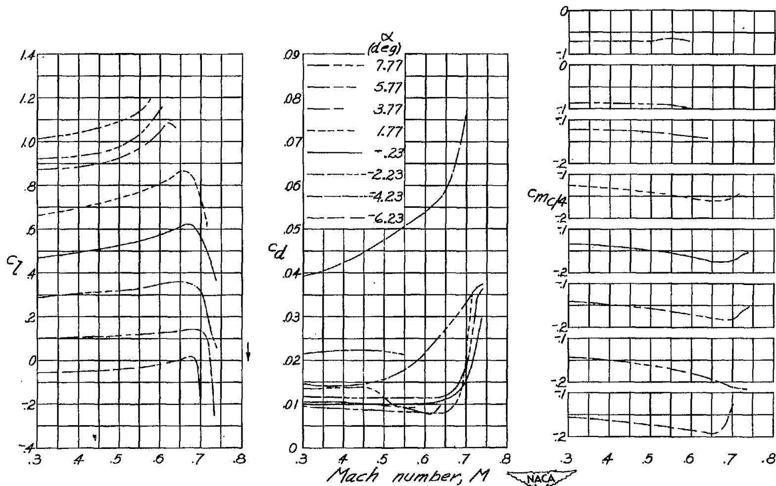
(4) NACA 16-712 airfoil. Figure 3.-Continued.
