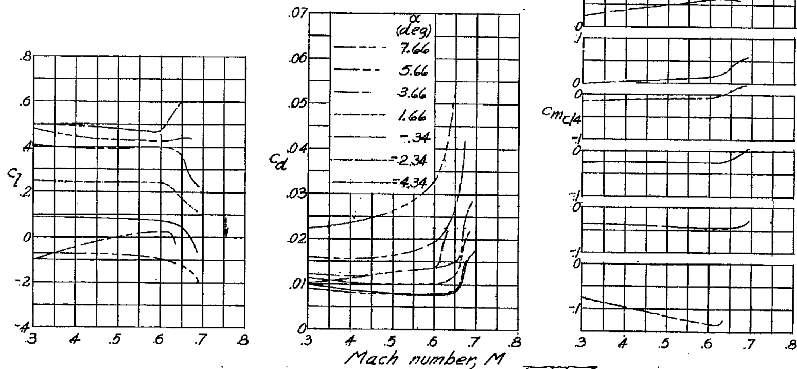
(1) NACA 16-321 airfoil. Figure 3.- Continued.
