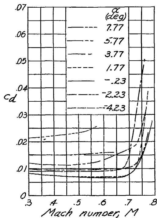
(p) NACA 16-512 airfoil. Figure 3-Continued.
