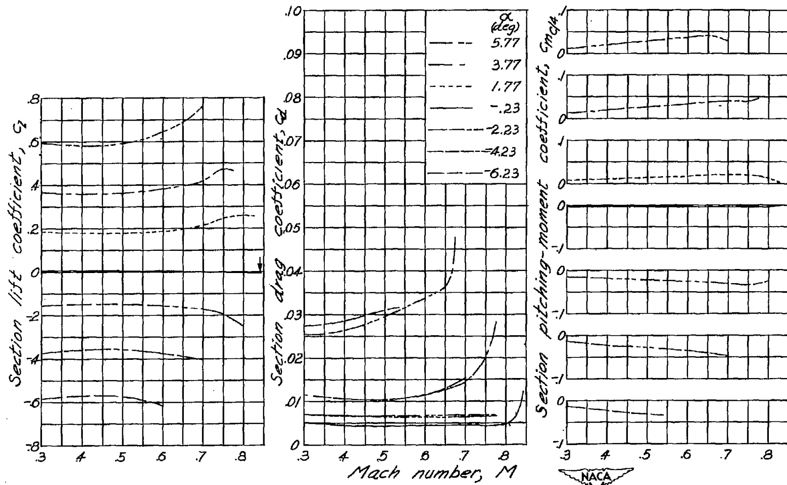
Figure 3.-Variation of airfoil section characteristics with Mach number.
