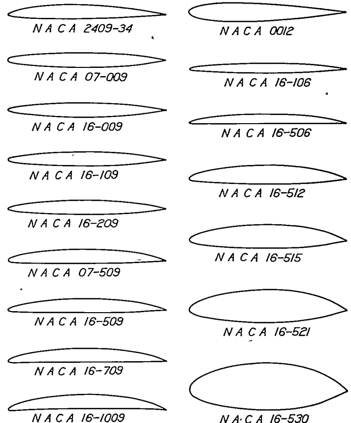
FIGURE 2.—Profiles for airfoils having high critical speeds.
