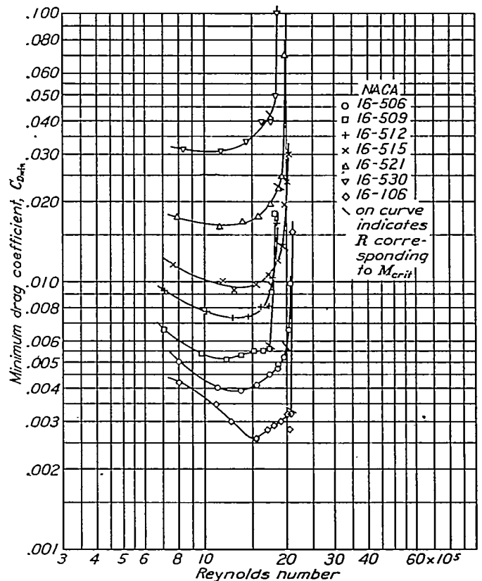
FIGURE 24.—Minimum drag for the NACA 16-500-series airfoils.
