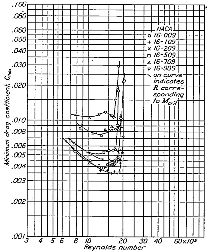
FIGURE 23.—Minimum drag for the NACA 16-009-series airfoils.
