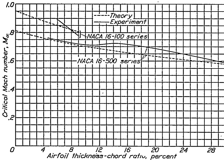
FIGURE 22.—Variation of airfoil critical Mach number with thickness-chord ratio.
