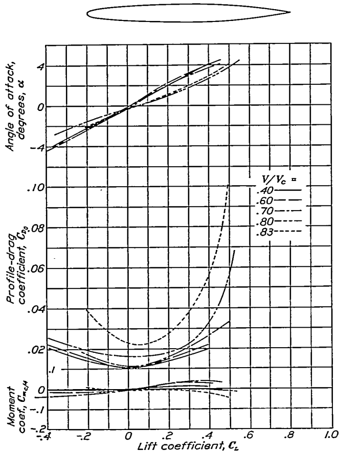
FIGURE 24.—Aerodynamic characteristics of the N.A.C.A. 0009-65 airfoil.
