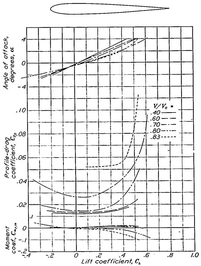
FIGURE 22.—Aerodynamic characteristics of the N.A.C.A. 0009-62 airfoil.
