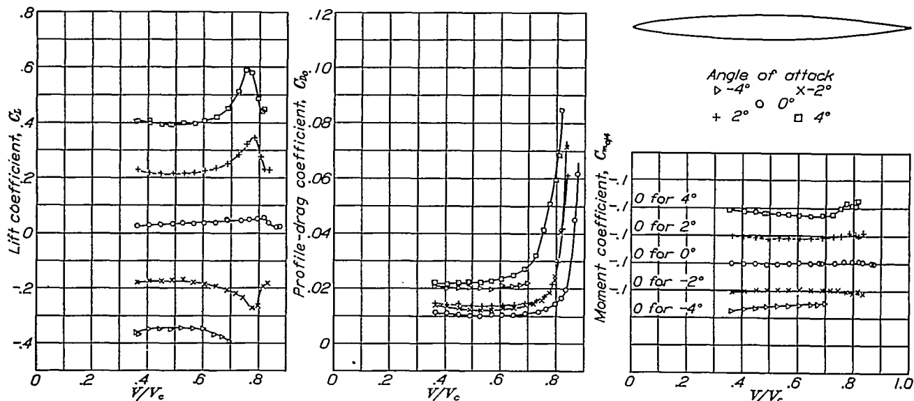
FIGURE 14.—Effect of compressibility on the aerodynamic characteristics of the N.A.C.A. 0009-35 airfoil.
