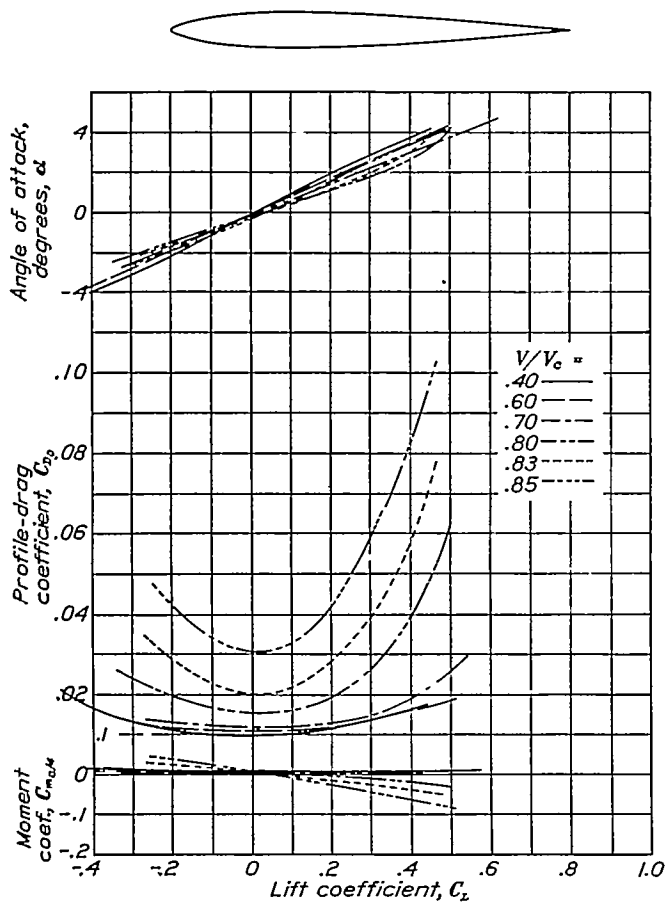
FIGURE 27.—Aerodynamic characteristics of the N.A.C.A. 0009-33 airfoil.
