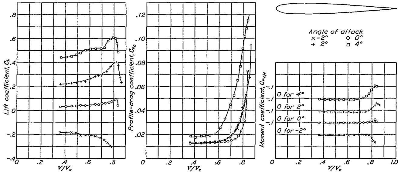
FIGURE 6.—Effect of compressibility on the aerodynamic characteristics of the N.A.C.A. 0009-62 airfoil.
