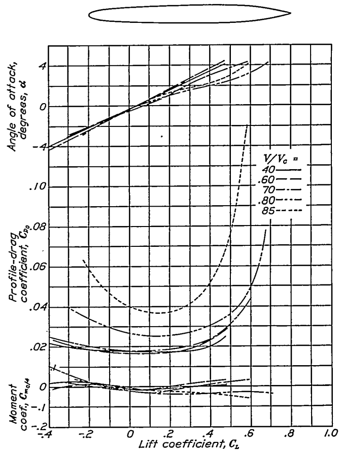
FIGURE 25.—Aerodynamic characteristics of the N.A.C.A. 0009-66 airfoil.
