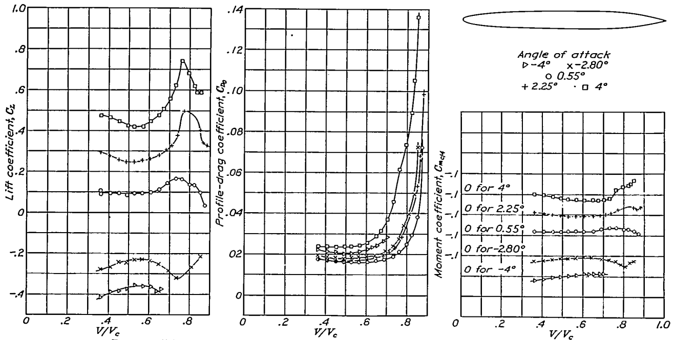
FIGURE 9.—Effect of compressibility on the aerodynamic characteristics of the N.A.C.A. 0009-60 airfoil.
