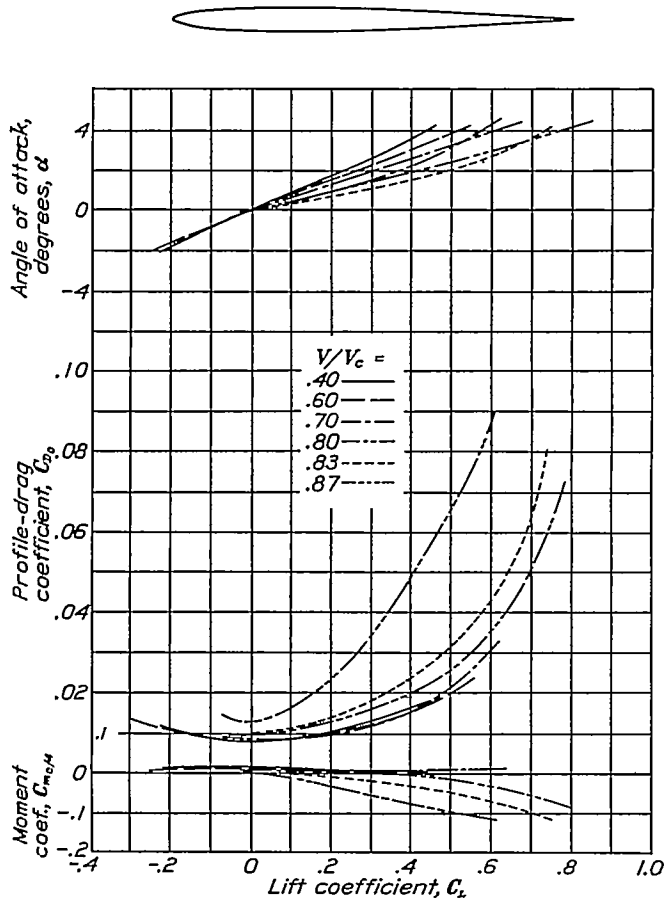
FIGURE 19.—Aerodynamic characteristics of the N.A.C.A. 0006-63 airfoil.
