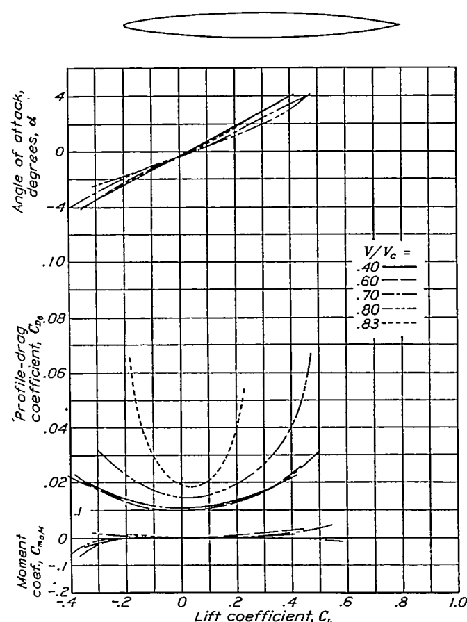
FIGURE 30.—Aerodynamic characteristics of the N.A.C.A. 0009-35 airfoil.
