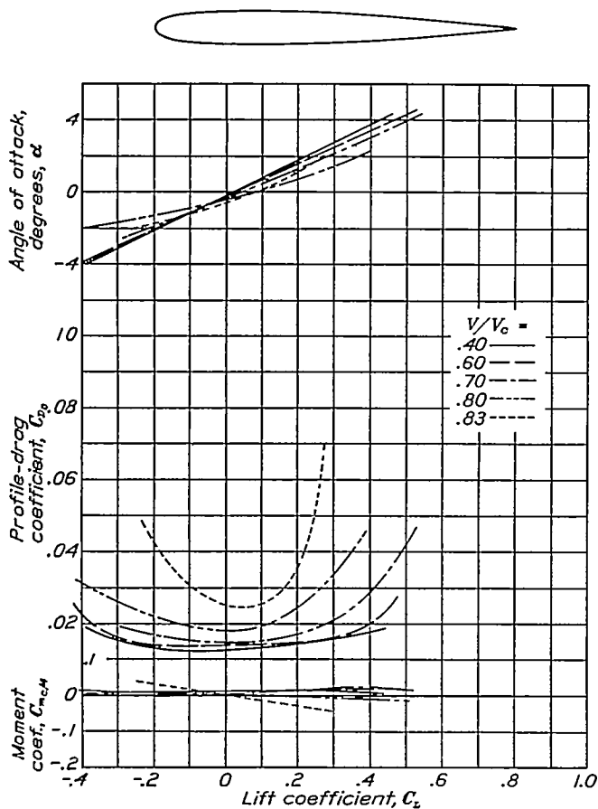
FIGURE 28.—Aerodynamic characteristics of the N.A.C.A. 0009-03 airfoil.
