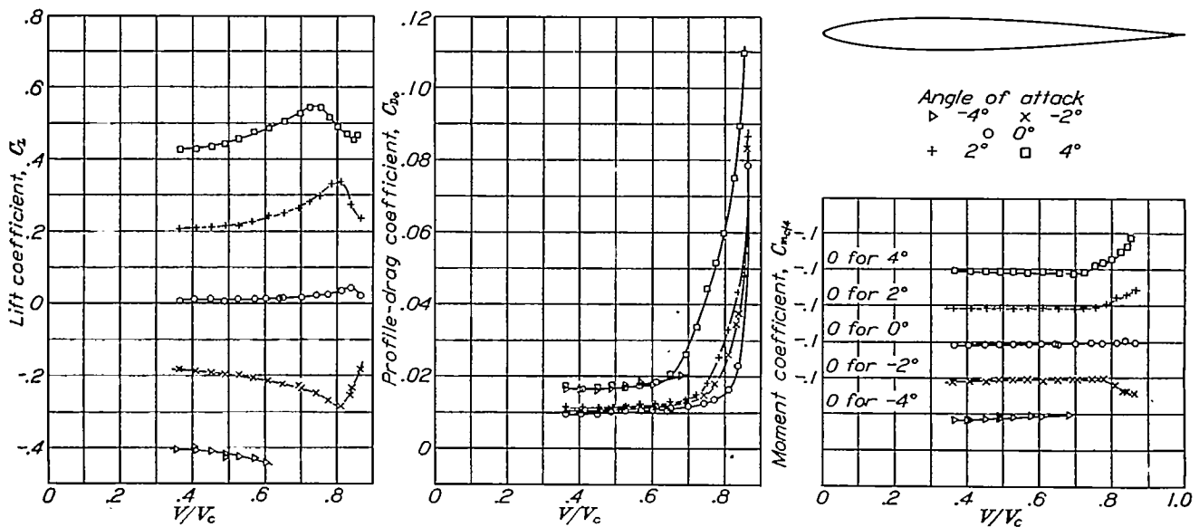
FIGURE 11.—Effect of compressibility on the aerodynamic characteristics of the N.A.C.A. 0009-33 airfoil.
