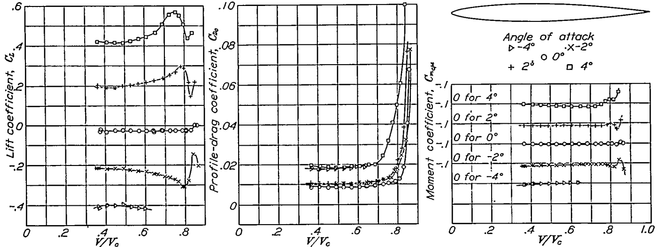
FIGURE 15.—Effect of compressibility on the aerodynamic characteristics of the N.A.C.A. 0009-34 airfoil.
