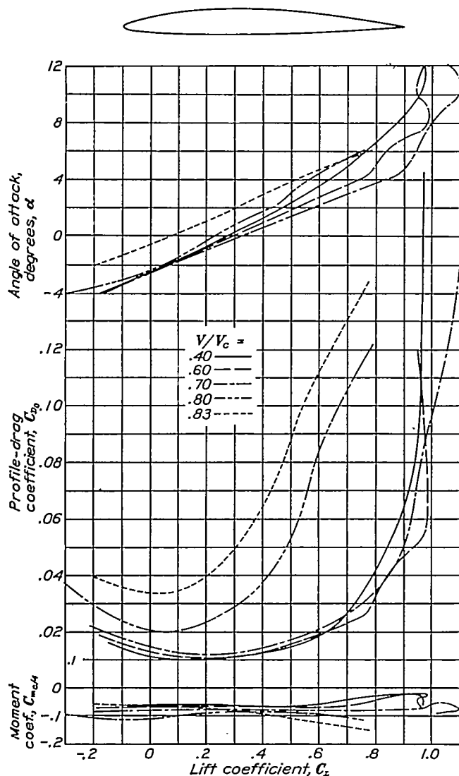
FIGURE 33.—Aerodynamic characteristics of the N.A.C.A. 2409-34 airfoil.
