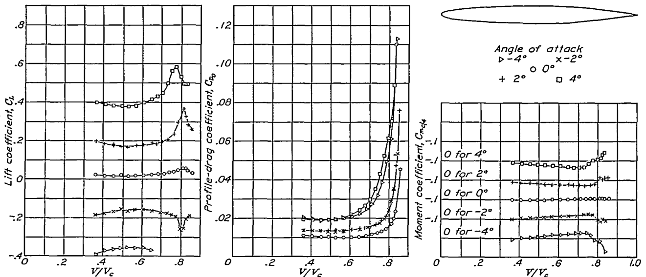
FIGURE 8.—Effect of compressibility on the aerodynamic characteristics of the N.A.C.A. 0009-65 airfoil.
