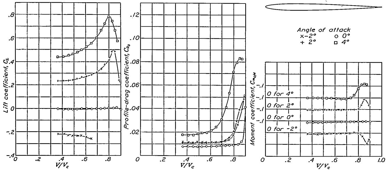
FIGURE 3.—Effect of compressibility on the aerodynamic characteristics of the N.A.C.A. 0006-63 airfoil.
