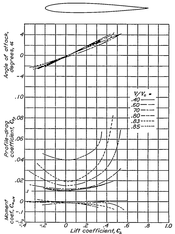
FIGURE 21.—Aerodynamic characteristics of the N.A.C.A. 0009-63 airfoil.
