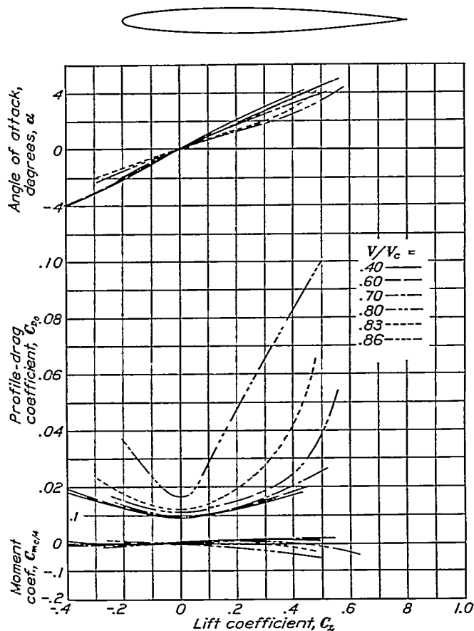
FIGURE 23.—Aerodynamic characteristics of the N.A.C.A. 0009-64 airfoil.
