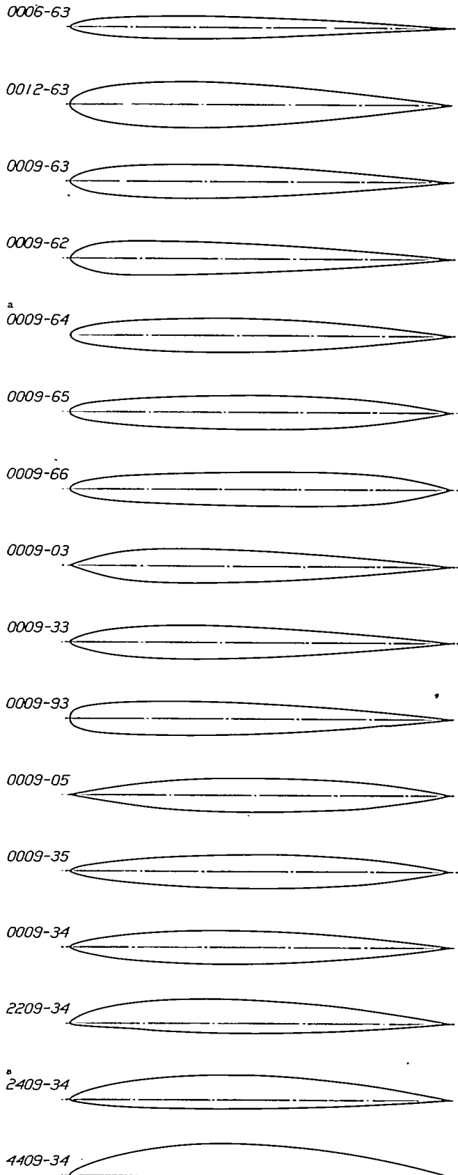
FIGURE 2.—Airfoil profiles.
