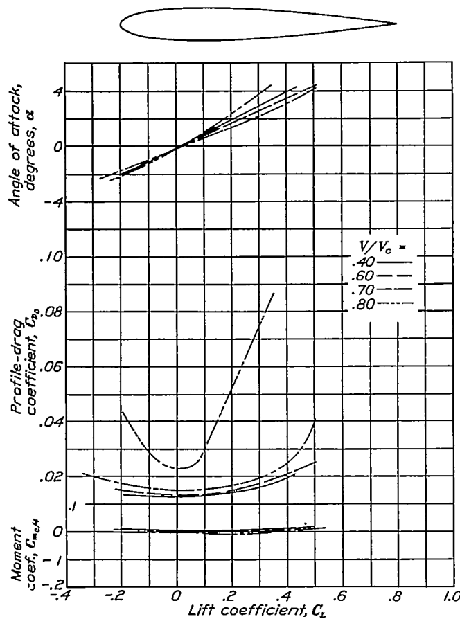
FIGURE 20.—Aerodynamic characteristics of the N.A.C.A. 0012-63 airfoil.
