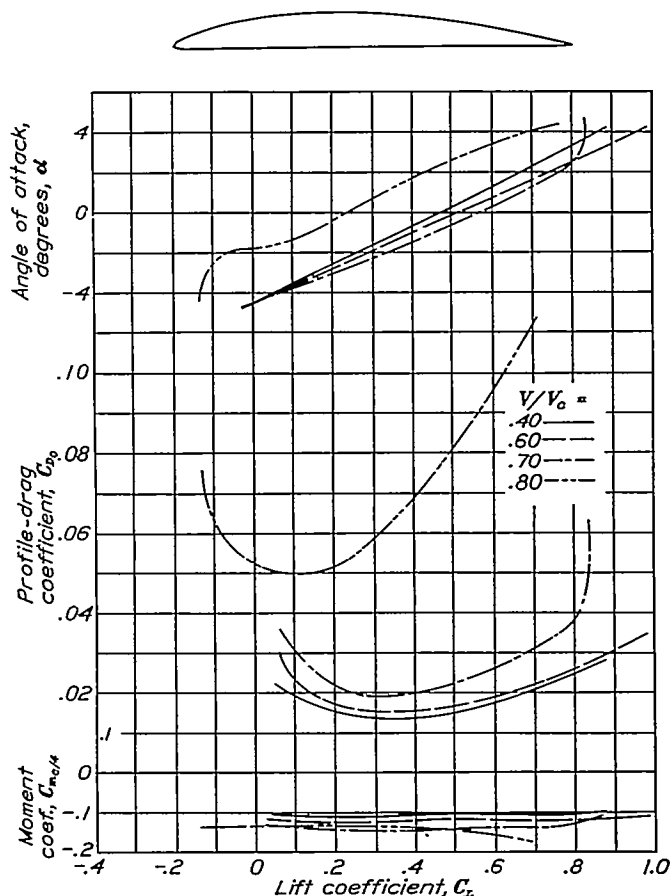
FIGURE 34.—Aerodynamic characteristics of the N.A.C.A. 4409-34 airfoil.
