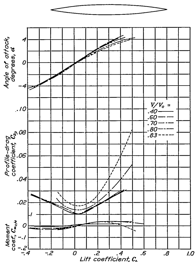
FIGURE 29.—Aerodynamic characteristics of the N.A.C.A. 0009-05 airfoil.
