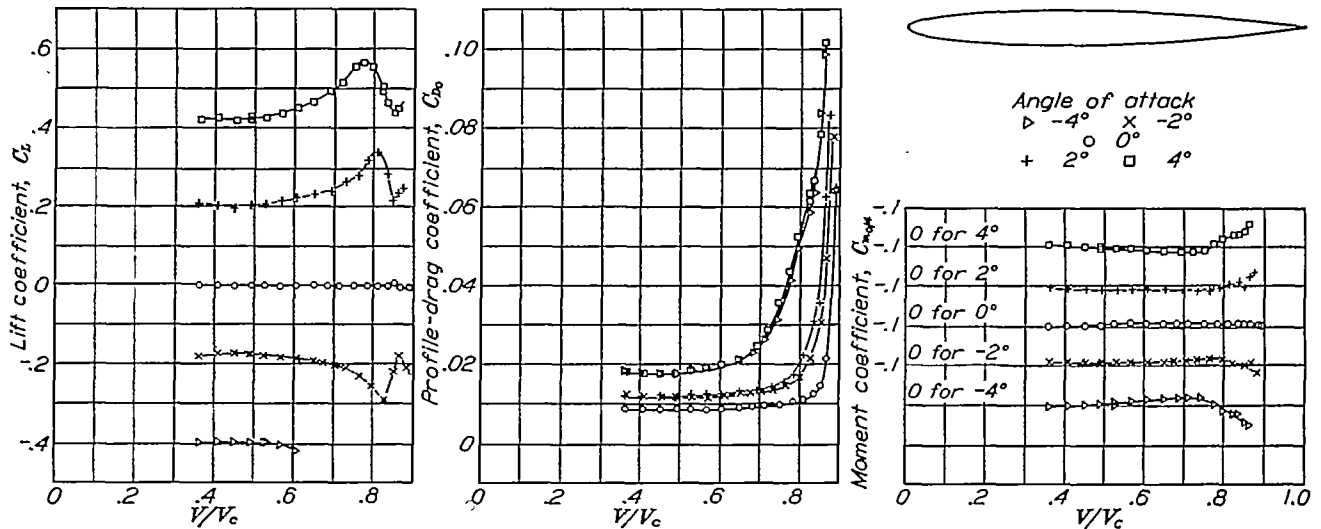
FIGURE 7.—Effect of compressibility on the aerodynamic characteristics of the N.A.C.A. 0009-64 airfoil.
