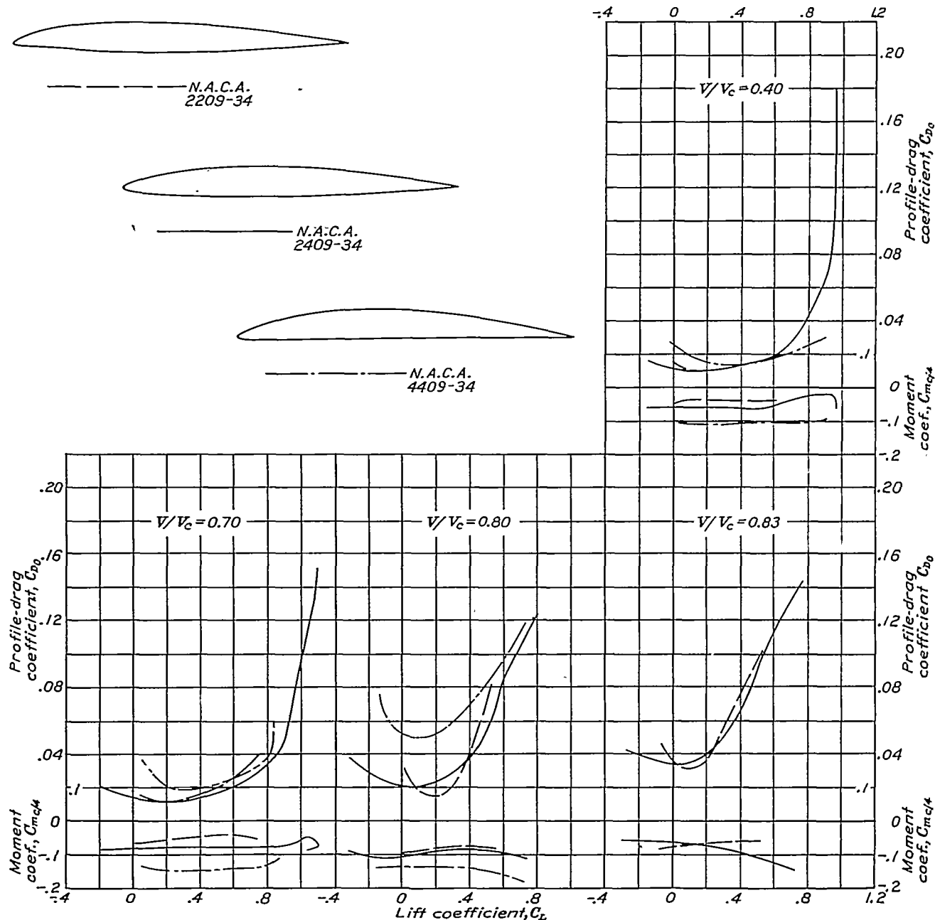
FIGURE 39.—Comparison of related cambered airfoils.
