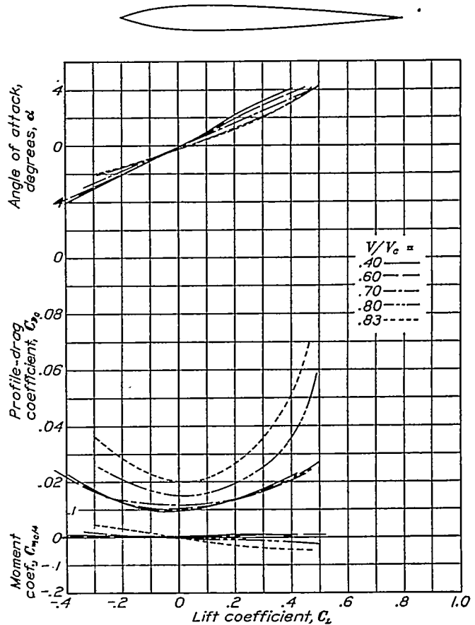
FIGURE 26.—Aerodynamic characteristics of the N.A.C.A. 0009-63 airfoil.
