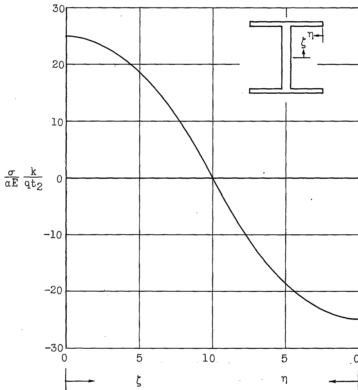
(a) H-section.
