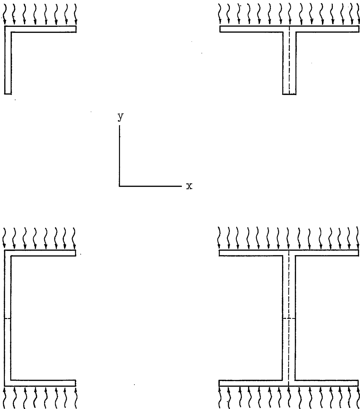
Figure 11.- Structural shapes formed by combinations of angle sections.
