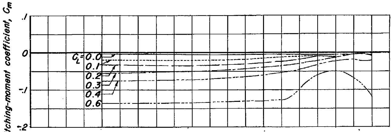
(a) Horizontal tail mounted in the extended wing-chord plane.
