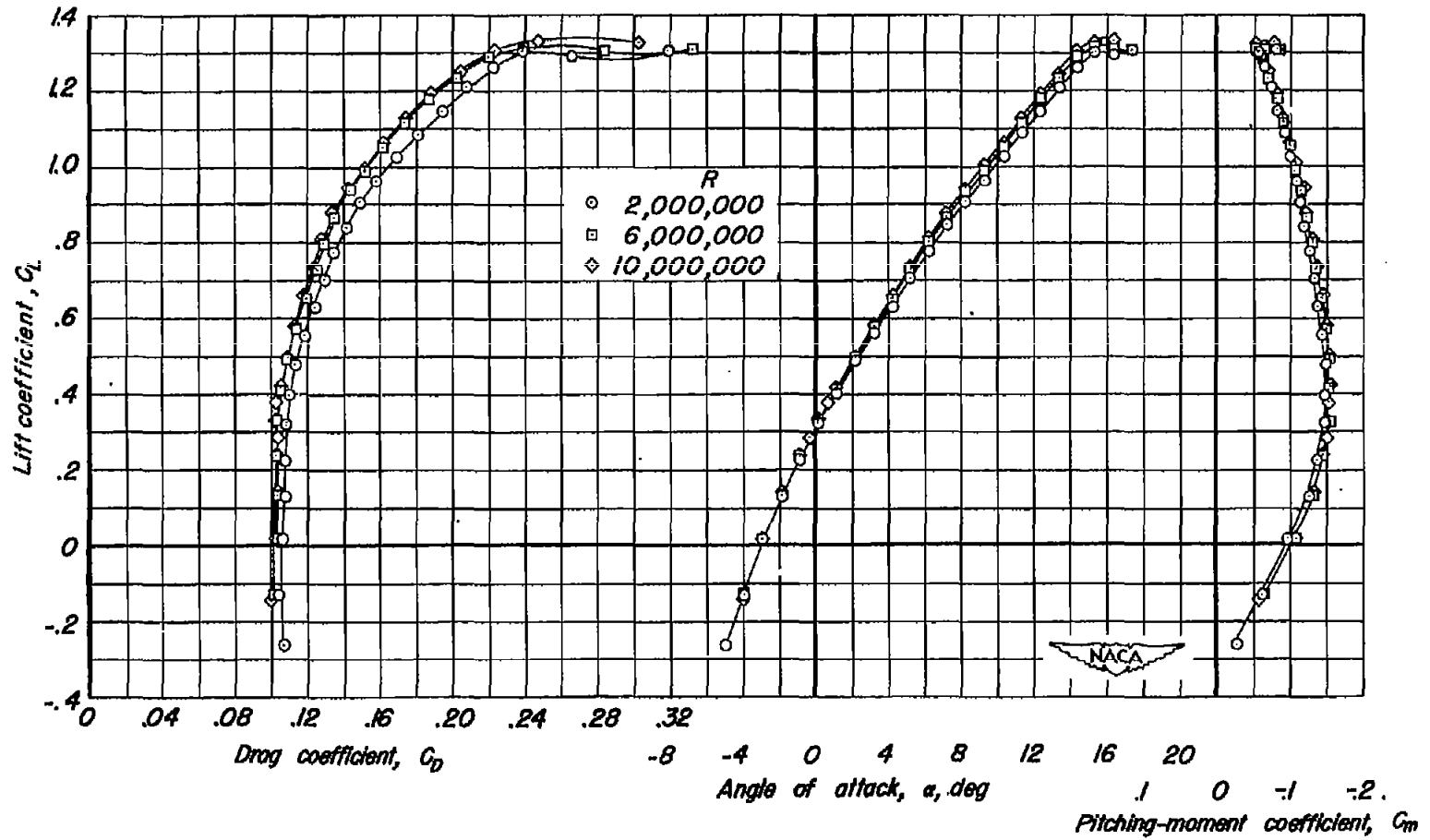
Figure 9.- The lift, drag, and pitching-moment characteristics of the wing and fuselage with the flaps deflected. \delta_f, 30^\circ ; \delta_f, 50^\circ ; M, 0.20 .
