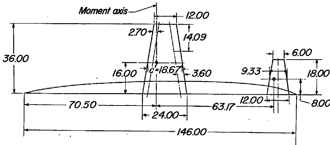
(a) Horizontal tail mounted in extended wing-chord plane.
