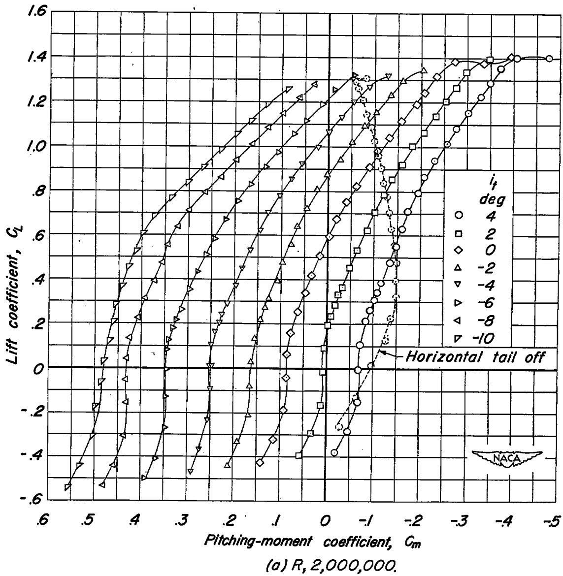
Figure 15.- The pitching-moment characteristics of the airplane model with the horizontal tail mounted in the extended wing-chord plane and with the flaps deflected. \delta_h, 30^\circ; \delta_f, 50^\circ; M, 0.20 .
