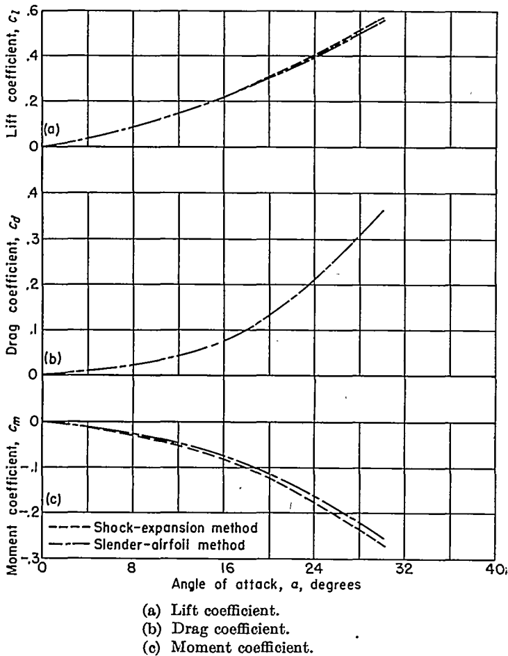
FIGURE 24.—Variation of force and moment coefficients with angle of attack for 10-percent-thick biconvex airfoil section at M_0=10 , T_0=500^\circ \text{ R} .
